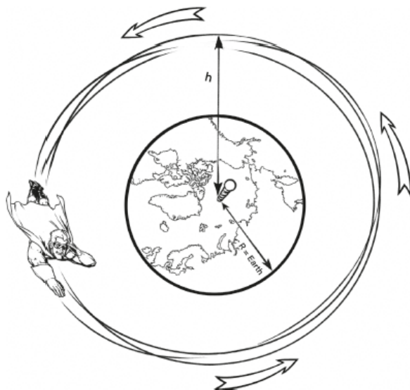
Figure 1: Sketch of Earth and our superhero CLPIP orbiting the planet. Earth's radius (labeled R_{\text{EARTH}} ) and the height of the orbiting hero h are indicated.
